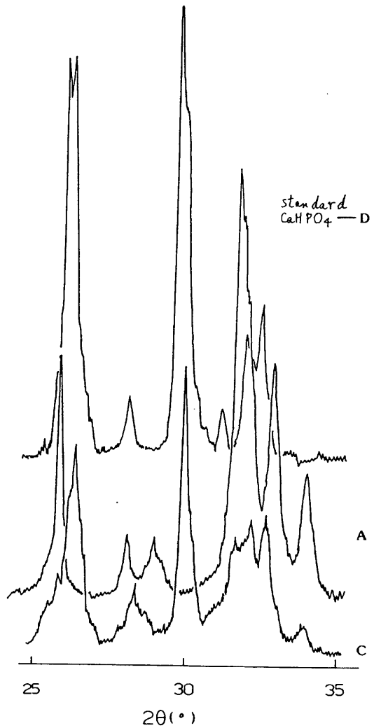
Fig. 2. X-ray powder diffraction patterns 6) of synthesized calcium phosphate (CuKα)
