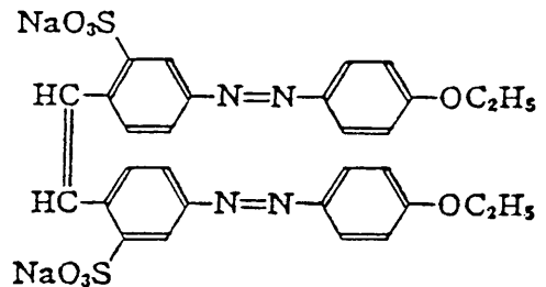
図1. C.I. Direct Yellow 12
