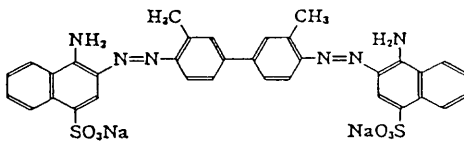
図4. C. I. Direct Red 2
