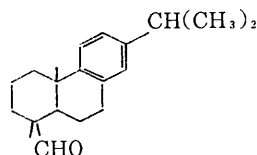
[1R-(1 \alpha , 2 \alpha\beta , 10 \alpha\alpha )]-7-(1-methylethyl)-1,2,3,4,4a,9,10,10a-octahydro-1,4a-dimethyl-1-phenanthrene-carboxaldehyde (dehydroabietal)
