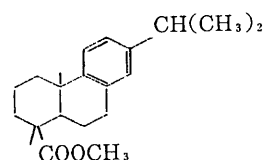
[1R-(1 \alpha , 4 \alpha\beta , 10 \alpha\alpha )]-7-(1-methylethyl)-1,2,3,4,4a,9,10,10a-octahydro-1,4a-dimethyl-1-phenanthrene-carboxylic acid methyl ester (methyldehydroabietate)
